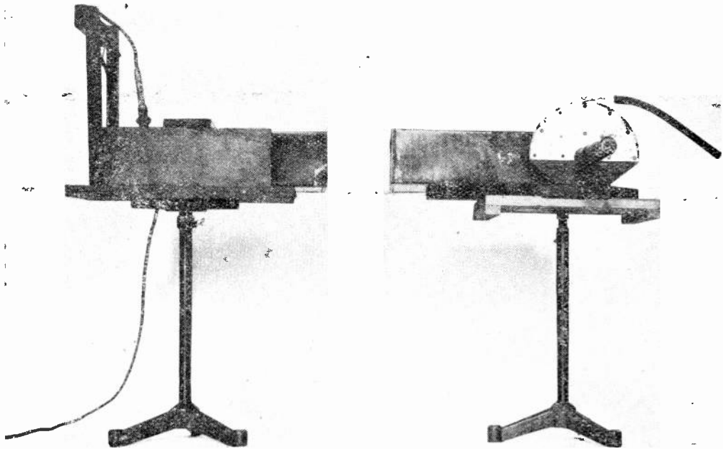
Fig. 62. General view of the Author's apparatus for showing experiments with short electric waves illustrating their similarity to light waves and the opacity or transparency of various substances.
