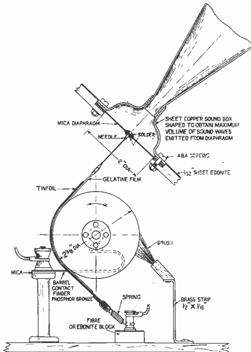
Fig. 1. Details of drum, band and diaphragm.
