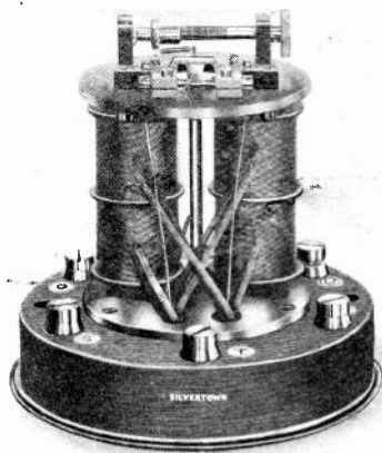
Fig. 60. A telegraph relay with outer case removed.
