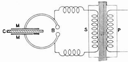
Fig. 50. Arrangement for producing electric oscillations.
