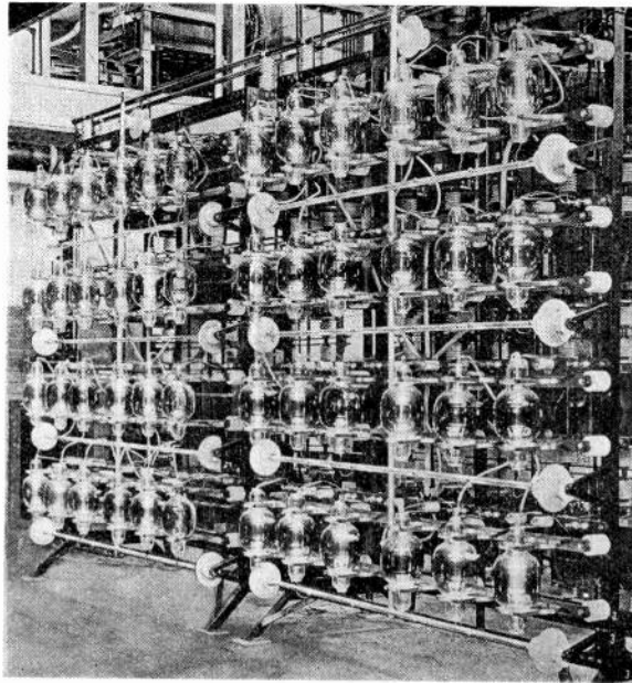
Fig. 71. Valve Transmitting Panel at Marconi Station near Carnarvon.
