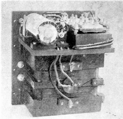
Interior view from the back, showing variometer stationary winding, cell, buzzer, and fixed value condensers. The sockets on the left are those to which leads are joined in converting the wavemeter for use on short wavelengths.
