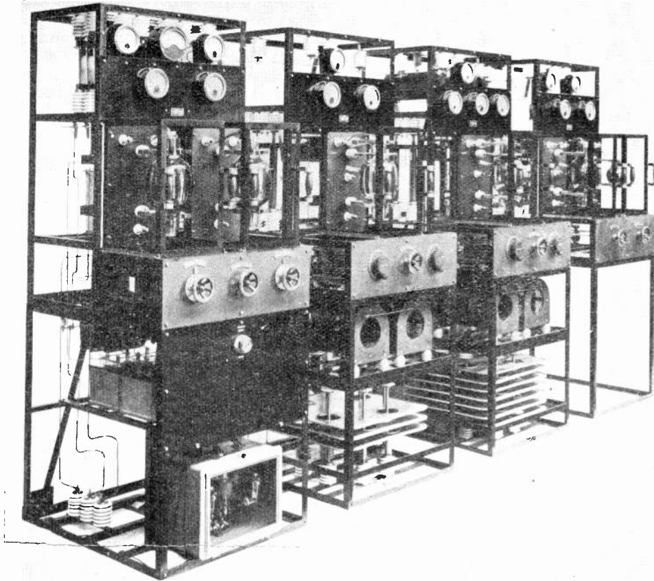
The Type of Transmitting Apparatus employed at the London Broadcasting Station.
