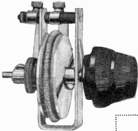
Type No. 11601/HI Filament Rheostat with Vernier Adjustment.
