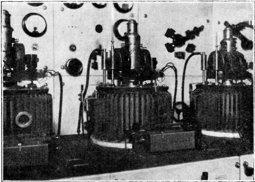
Fig. 10. Mercury circuit breakers, which interrupt the excitation current of the Alternator for signalling. The gap, which is ordinarily \frac{3}{8} -inch, may be varied between limits without interrupting transmission.
