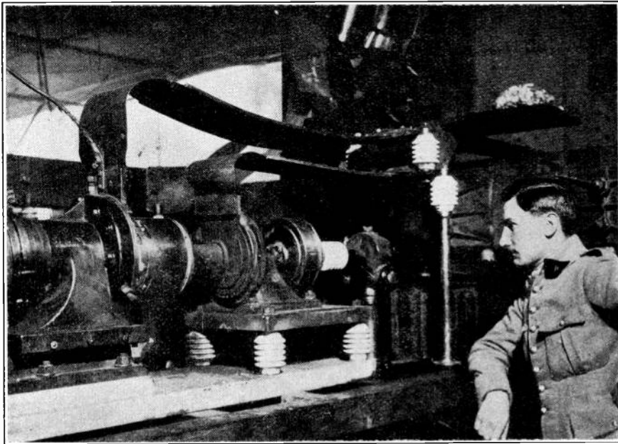
Fig. 7. Spark-Gap, with revolving eccentric electrode.
