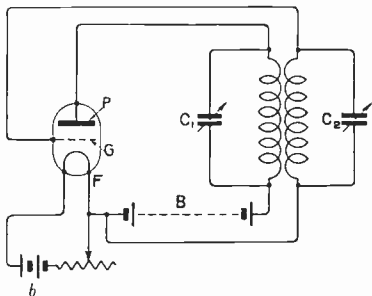
Fig. 70. Method of using a Thermionic Valve to create undamped electric oscillations. P. Plate of valve. G. Grid. F. Filament. B. Plate battery. b. Filament battery.
