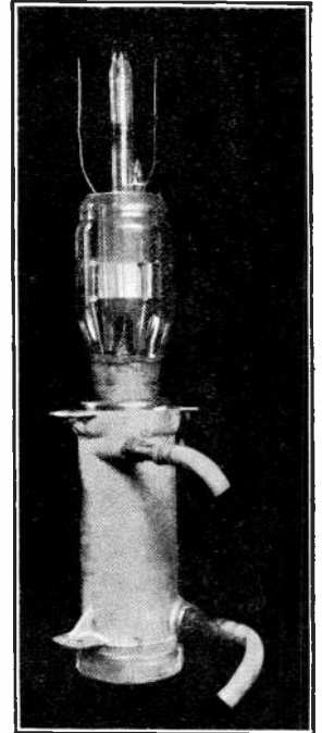
ABOVE: Valve inserted in water circulated cooling jacket.
